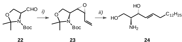
Scheme 8 Serinal-derived vinyloxirane 23 as a precursor for the synthesis of sphingoid bases. i) \gamma -( Z )-chloroallyl \text{B}(\text{Ipc})_2 , 8-hydroxyquinoline, DBU, ii) \text{C}_{12}\text{H}_{25}\text{CuCN} , hydrolysis.
