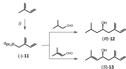
Scheme 4 Stereoselective one-pot synthesis of ipsenol ( R )- 12 and ipsdienol ( S )- 13 ; i ): n -BuLi, TMPK, -78\text{ }^{\circ}\text{C} , \text{dIpc}_2\text{BOMe} , \text{BF}_3 \cdot \text{OEt}_2 ; (TMPK: potassium 2,2,5,5-tetramethylpiperidide)
